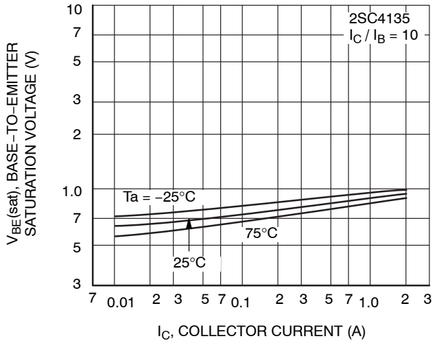
Figure 15. V_{BE(sat)} - I_C
